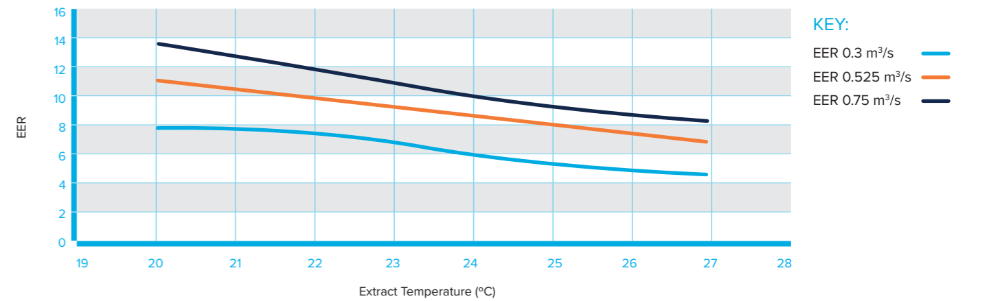
SIZE 07 PRE-COOLING MODE EER AT 35°C INTAKE
