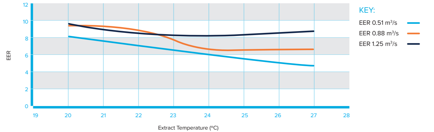
SIZE 12 PRE-COOLING MODE EER AT 35°C INTAKE
