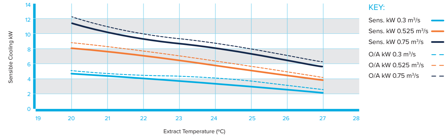
SIZE 07 PRE-COOLING MODE SENSIBLE/OVERALL KW OUTPUT AT 35°C INTAKE
