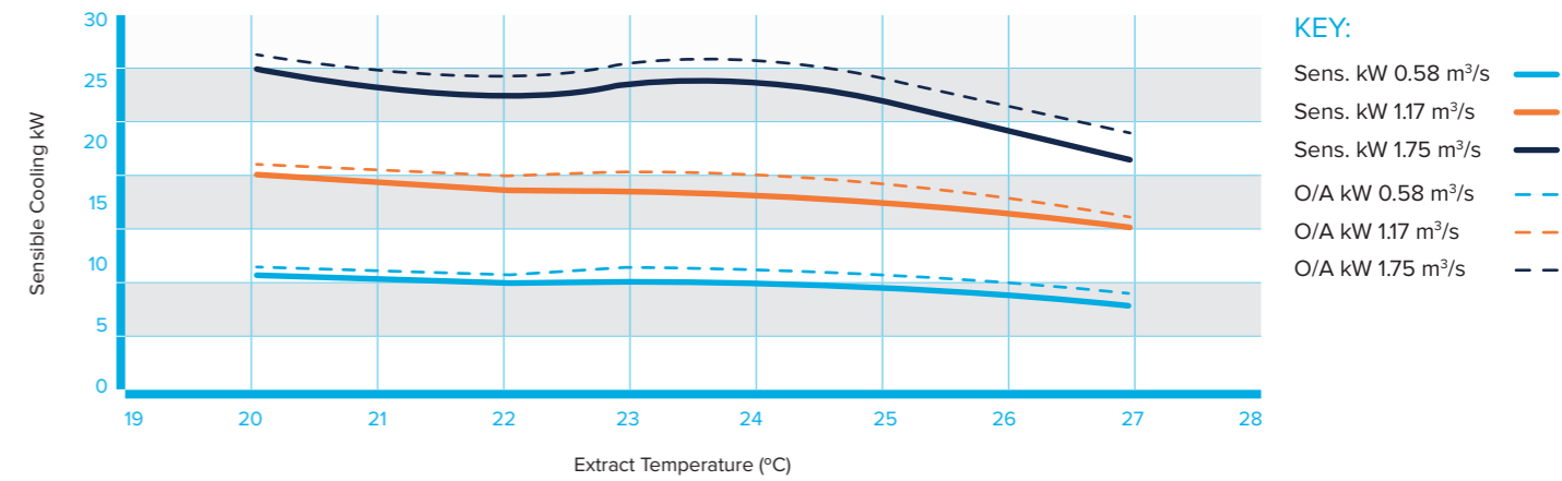
SIZE 17 PRE-COOLING MODE SENSIBLE/OVERALL KW OUTPUT AT 35°C INTAKE
